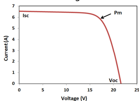
Fig 1: Current-voltage curve of a 100 W / 36 cell solar panel
