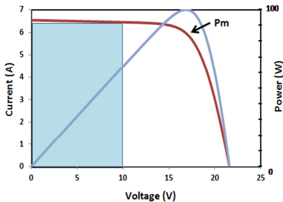
Fig 4: Less power harvested: voltage is too low
