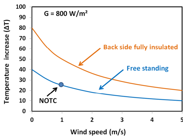
Fig 17: Wind speed and temperature increase
