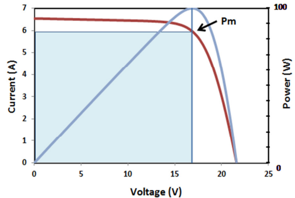
Fig. 3: The surface of the blue rectangle is proportional to the product P_m = V_m \times I_m
