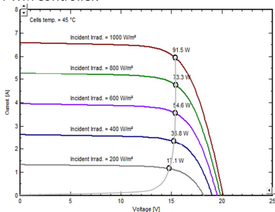
Figure 16: Dependence of M_p and V_{mp} on irradiance
